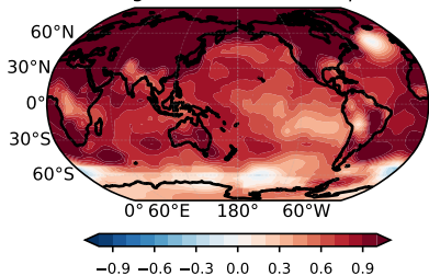
A Regression Coefficient ( \beta )
