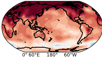
D \hat{y} = \beta(\bar{x}_t) + \alpha
