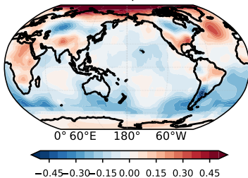
B Intercept ( \alpha )
