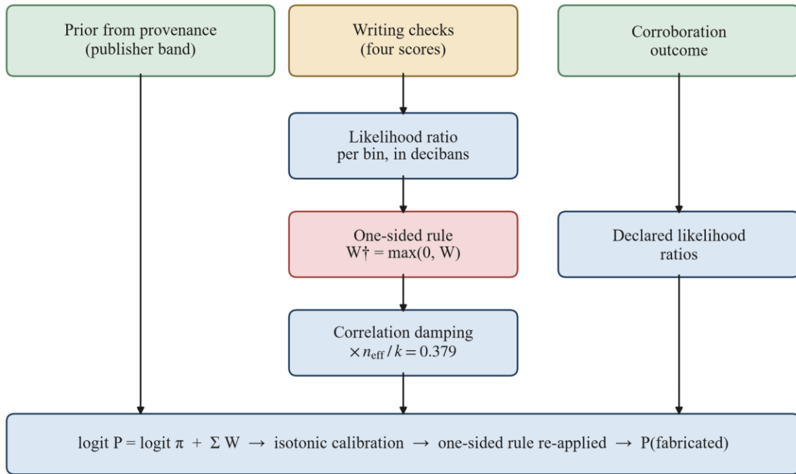
Figure 4.4 Scoring Model
