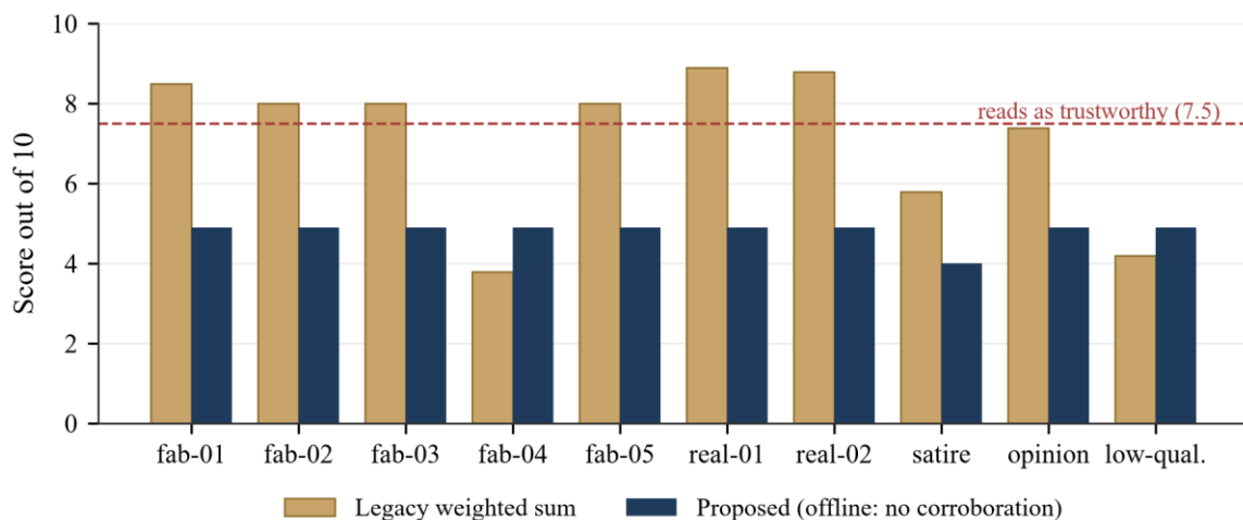
Figure 5.4 Scores of the Adversarial Items
