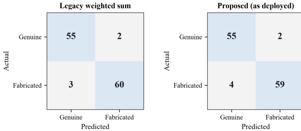
Figure 5.1 Confusion Matrices on the Held-out Set
