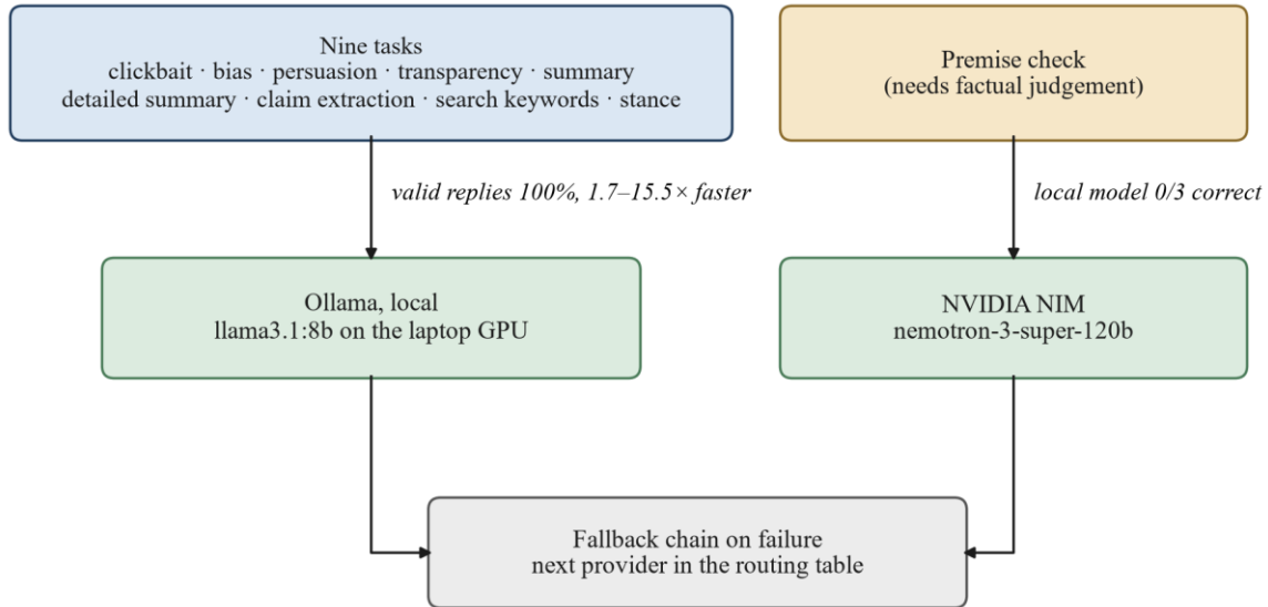
Figure 4.6 Task Routing Between Local and Hosted Models
