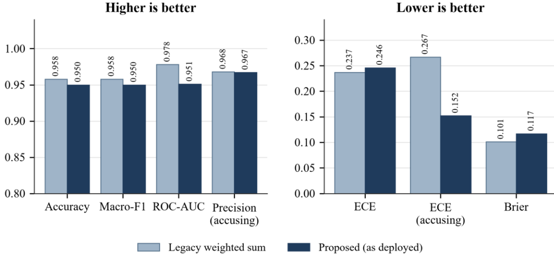
Figure 5.2 Comparison of Evaluation Metrics
