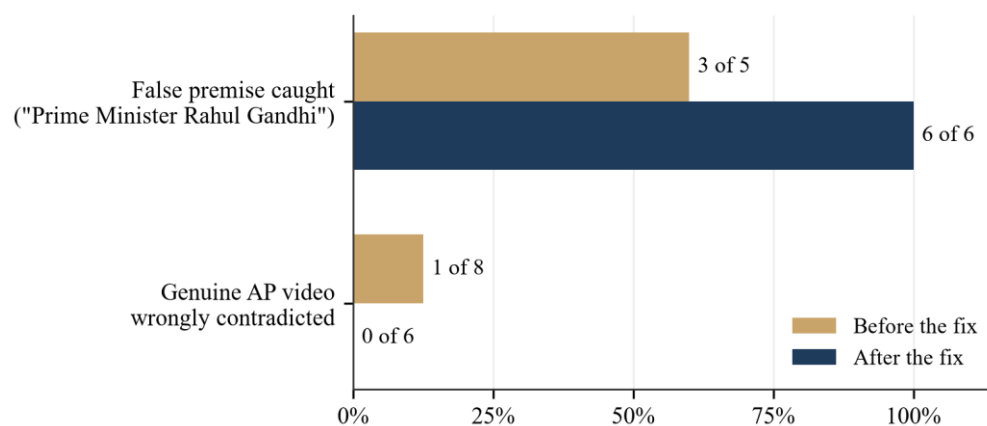
Figure 5.5 Premise Check Before and After the Corrections
