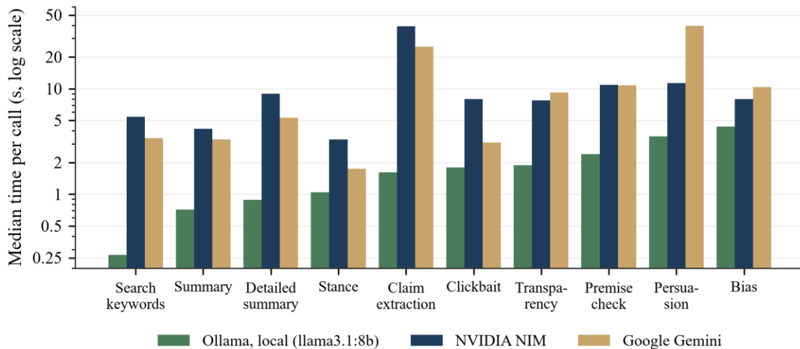
Figure 5.6 Median Time per Call by Provider
