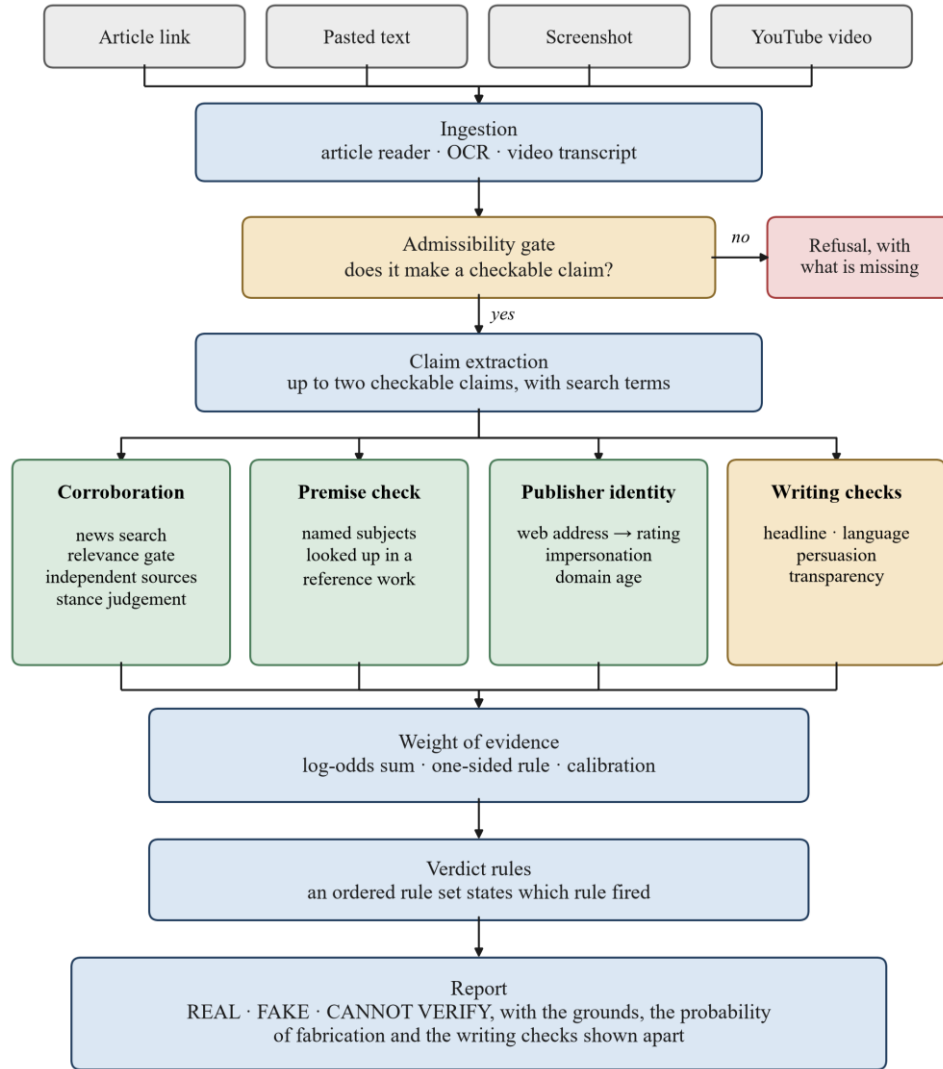
Figure 4.1 Proposed Approach
