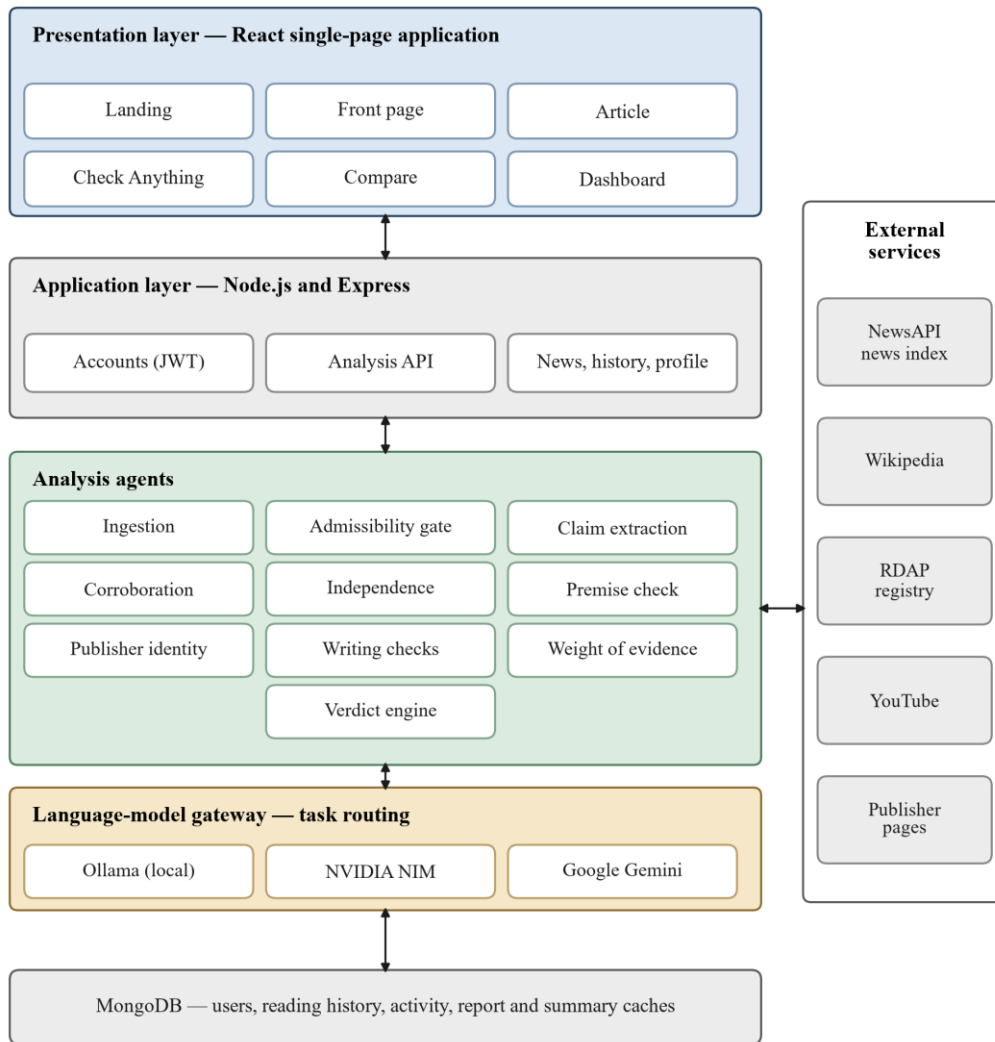
Figure 4.2 System Architecture
