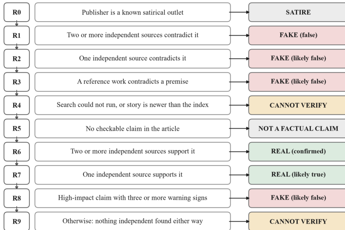
Figure 4.5 Verdict Rules in Order of Precedence
