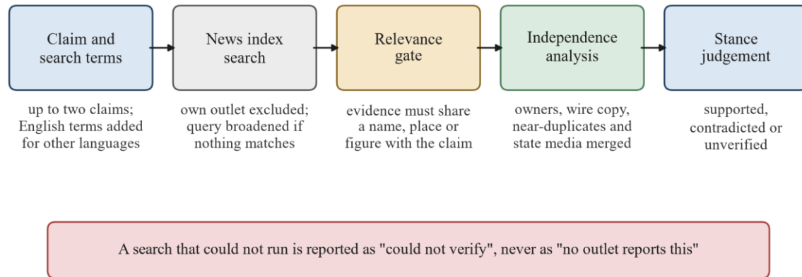
Figure 4.3 Corroboration Channel
