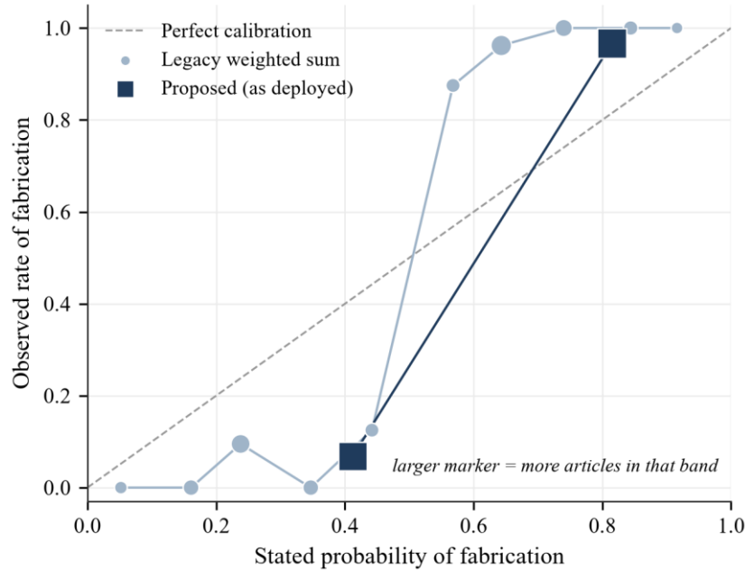
Figure 5.3 Reliability Diagram
