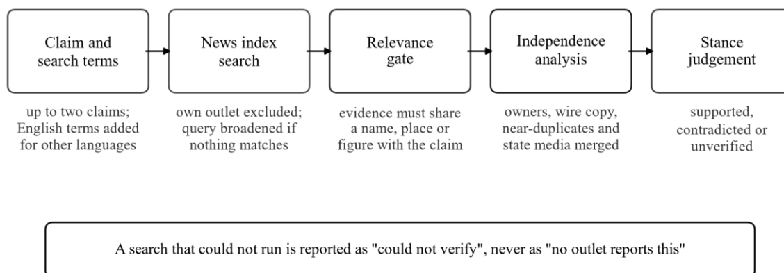
Figure 4.3 Corroboration Channel
