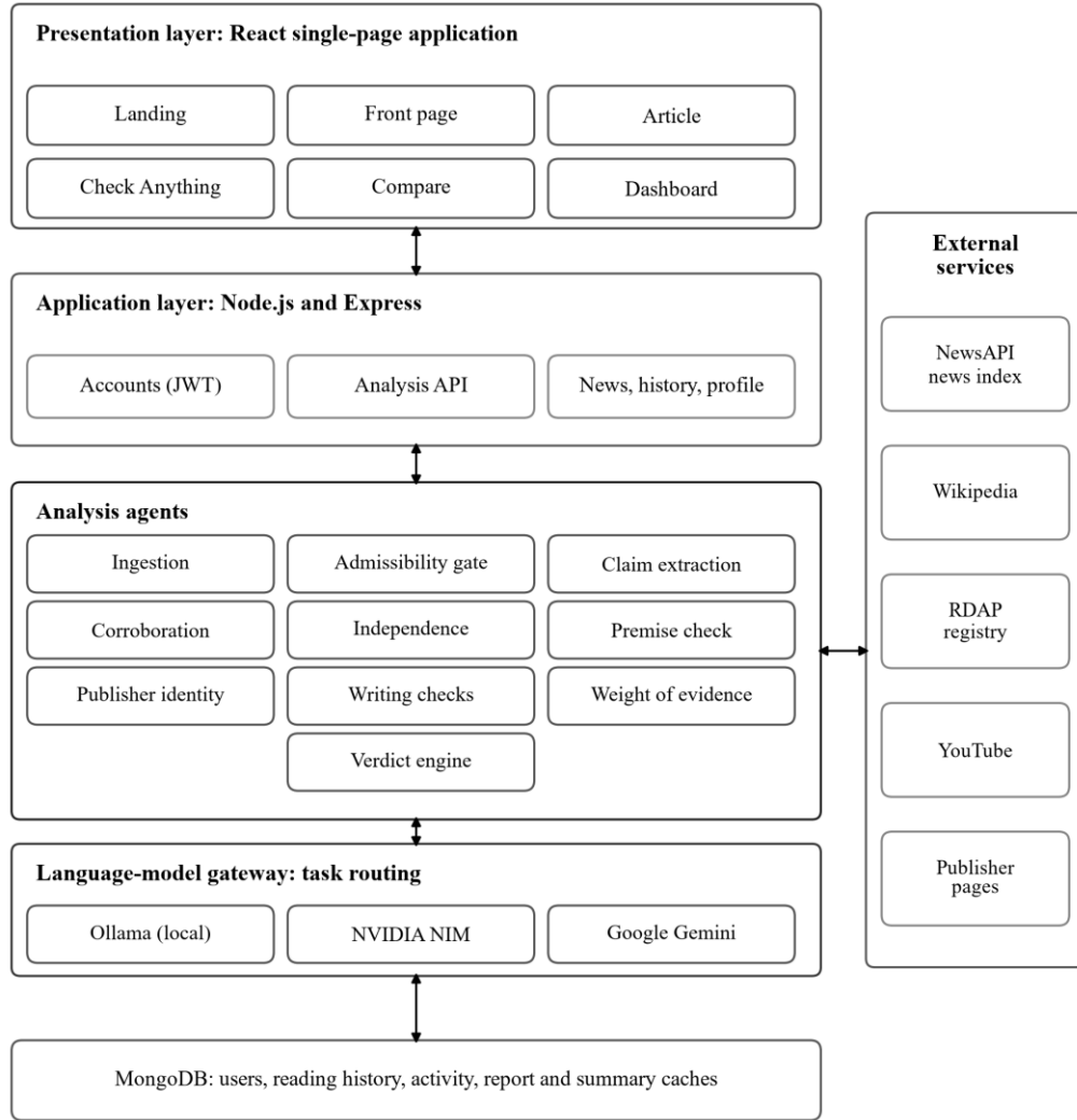
Figure 4.2 System Architecture
