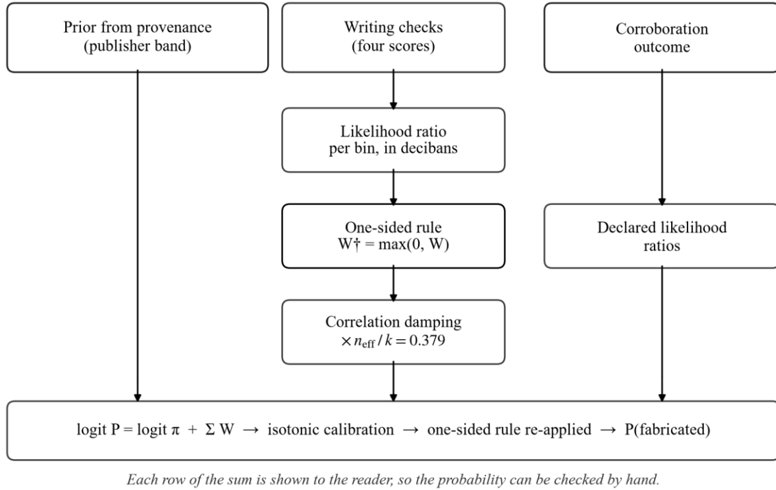
Figure 4.4 Scoring Model
