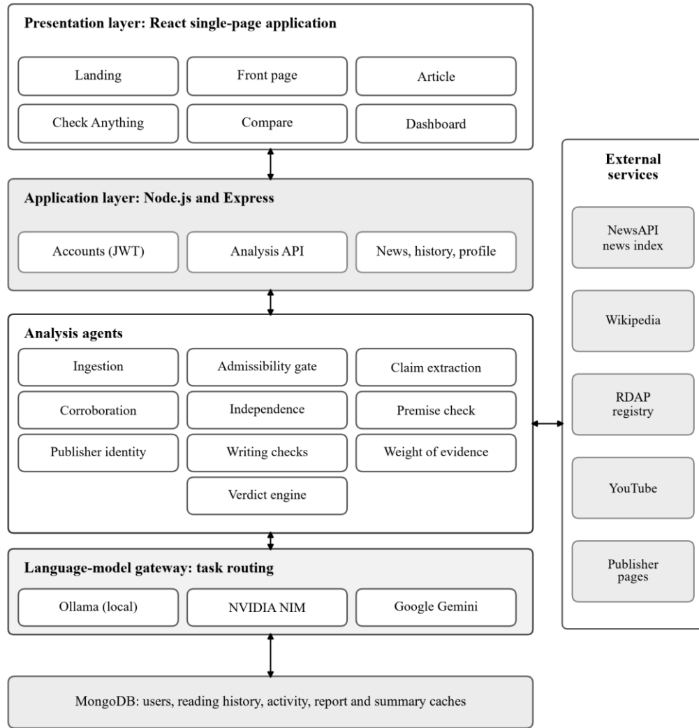
Figure 4.2 System Architecture
