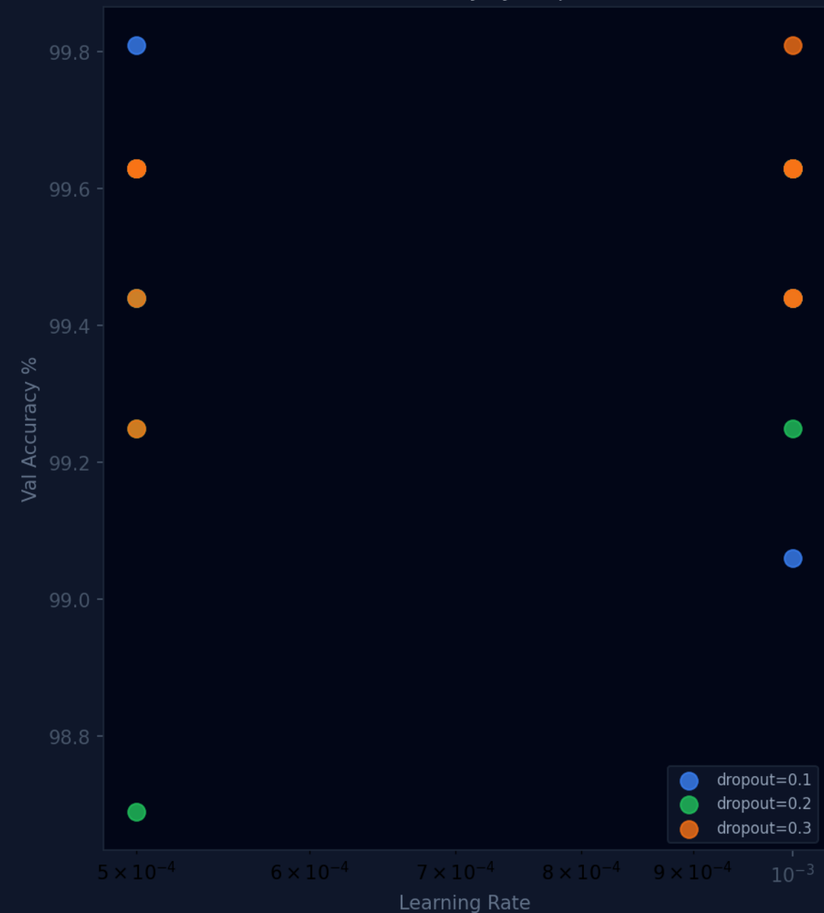
LR vs Accuracy by Dropout
