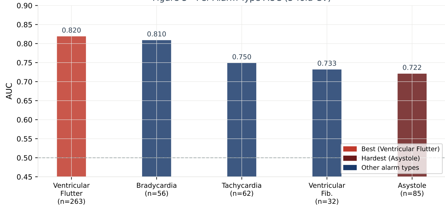
Figure 5 - Per-Alarm-Type AUC (5-fold CV)
