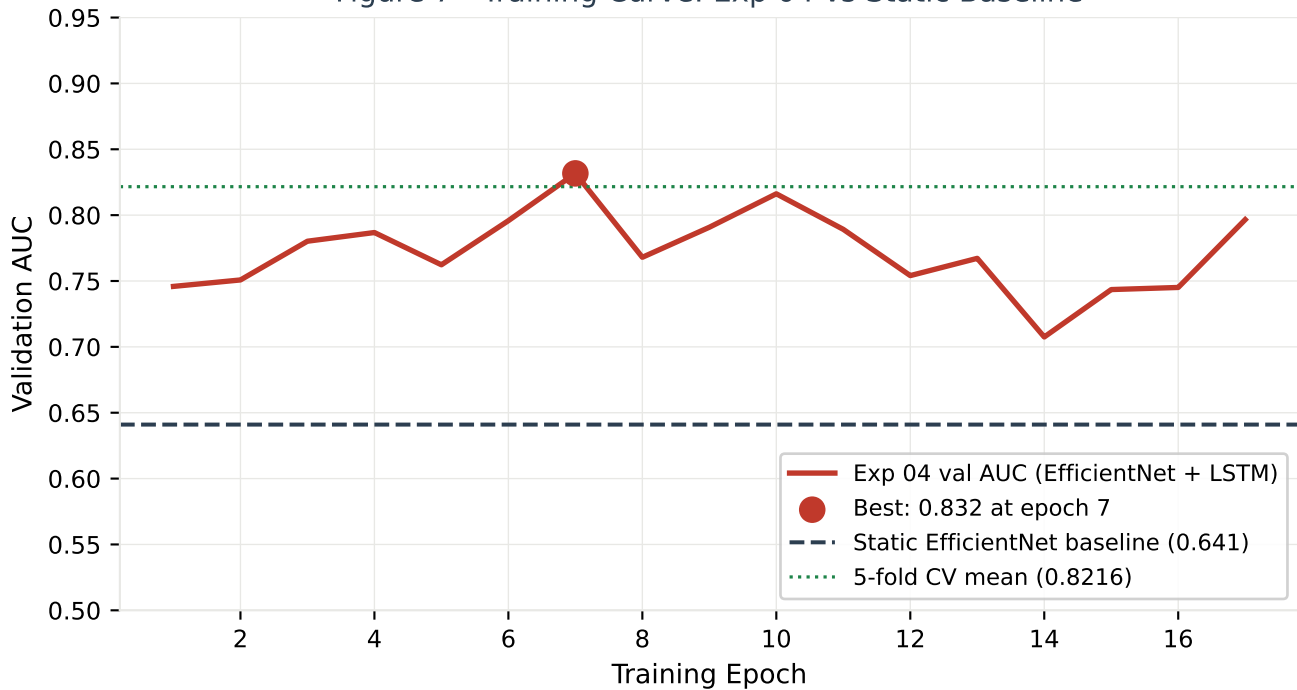
Figure 7 - Training Curve: Exp 04 vs Static Baseline
