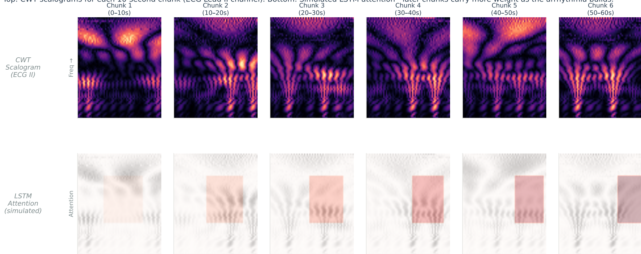
Figure 8 - Temporal Chunking: Record v101I (True Ventricular Flutter Alarm)
