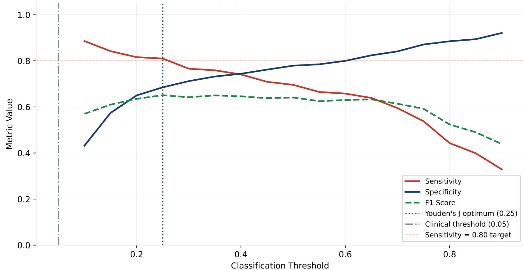
Figure 10 - Sensitivity, Specificity and F1 vs Classification Threshold
