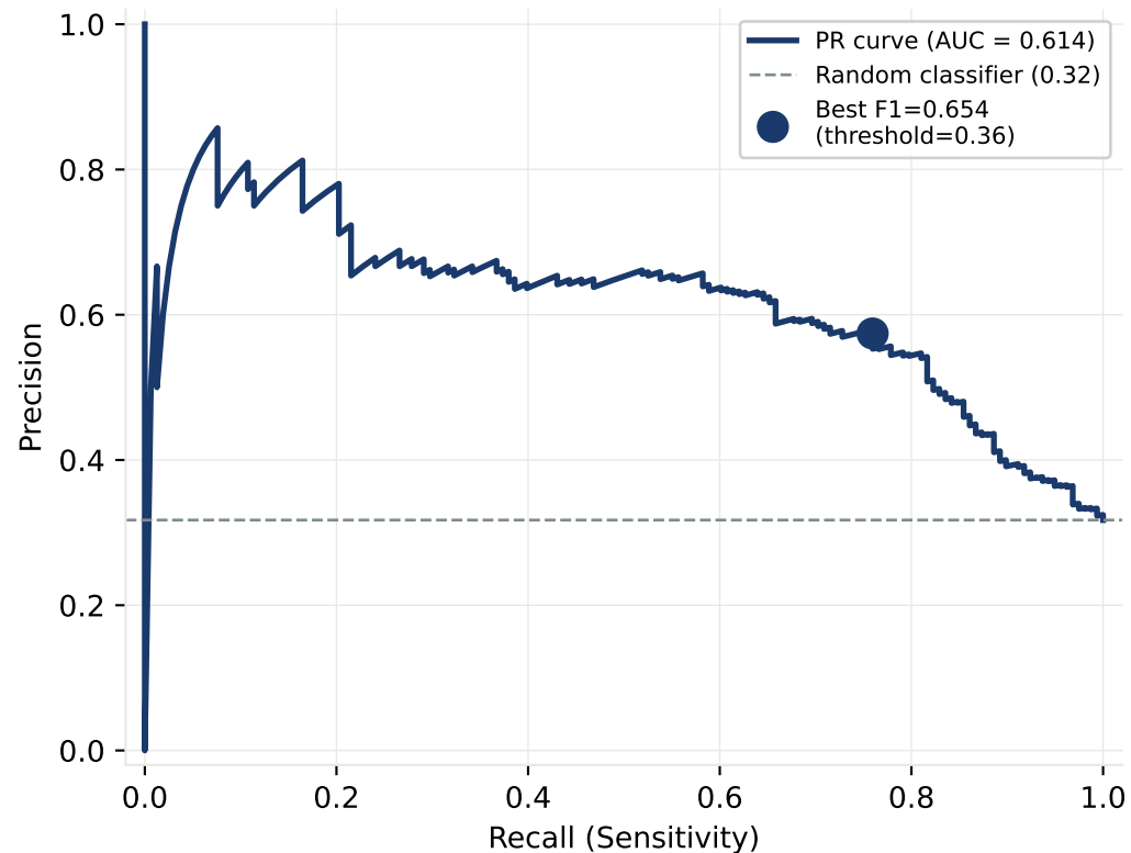
(b) Precision-Recall Curve - Experiment 04 EfficientNet + LSTM (5-fold OOF)
