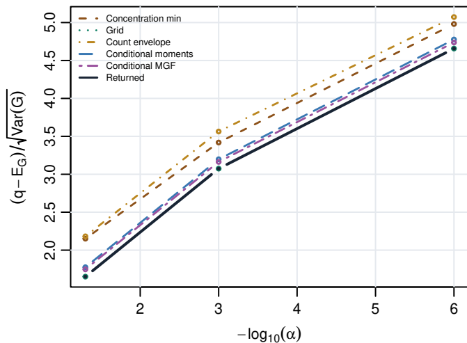
Square roots, unequal probabilities
