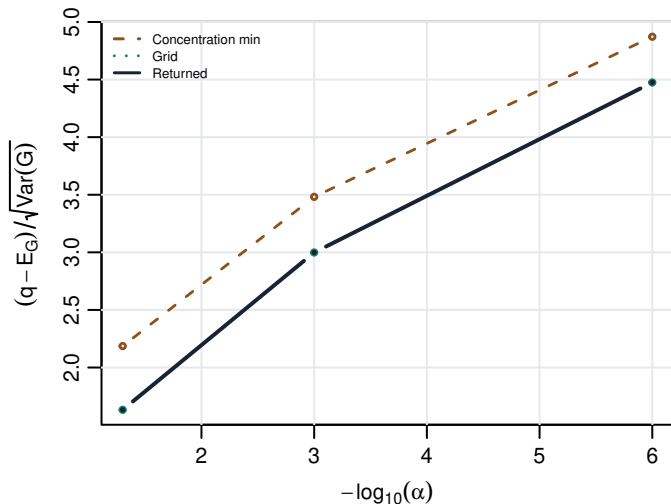
Square roots, unequal probabilities
