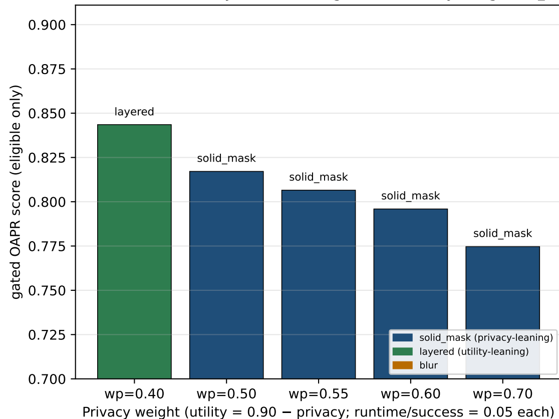
OAPR progressive evaluation — gated deployment selection (exploratory composites retained for comparison) A. Face anonymisation gated eligible winner by weight, low_step, falco, null, multi-modal paired scores, (stricter ≠ worse system)
