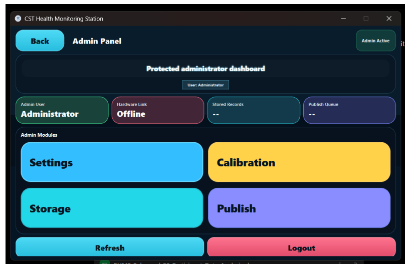
Figure 6.4: Admin Panel
