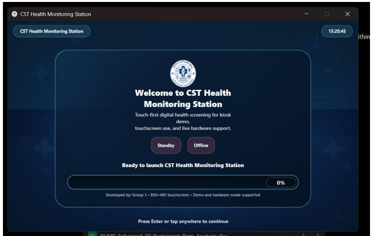
Figure 6.7: Welcome Screen
