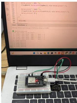
Figure 24: Testing of MAX301202
