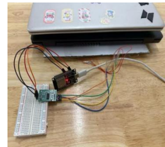
Figure 20: Testing of HX711 with load cell
