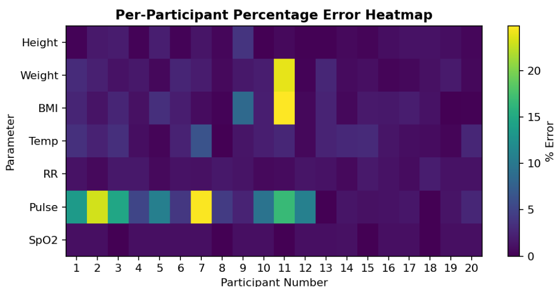
Figure 8.10: Per-participant percentage error heatmap
