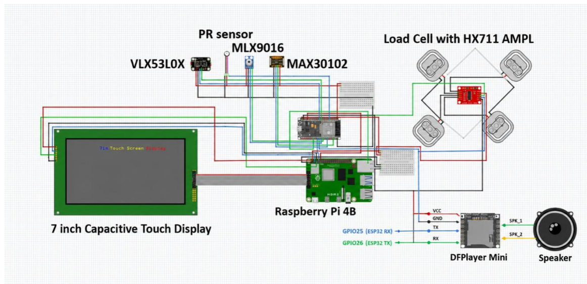
Figure 4.1: Circuit diagram showing capacitive touch display, Raspberry Pi 4B, ESP32, sensors, and load cell with HX711 amplifier connections.
