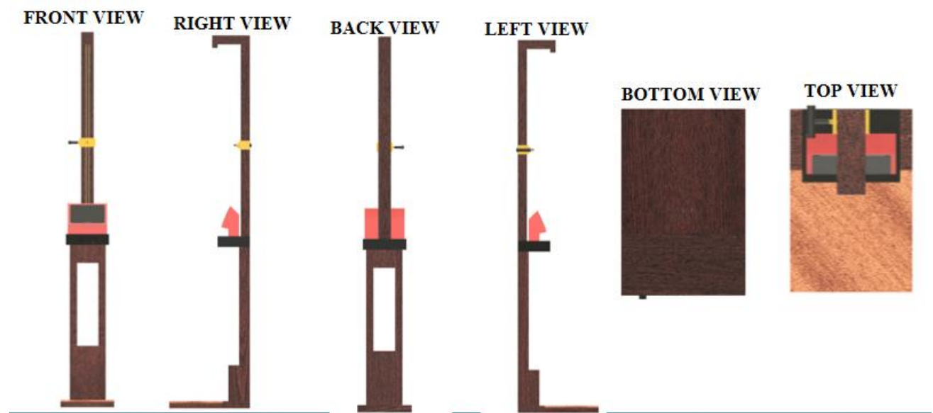
Figure 12: Views of 3D Design
