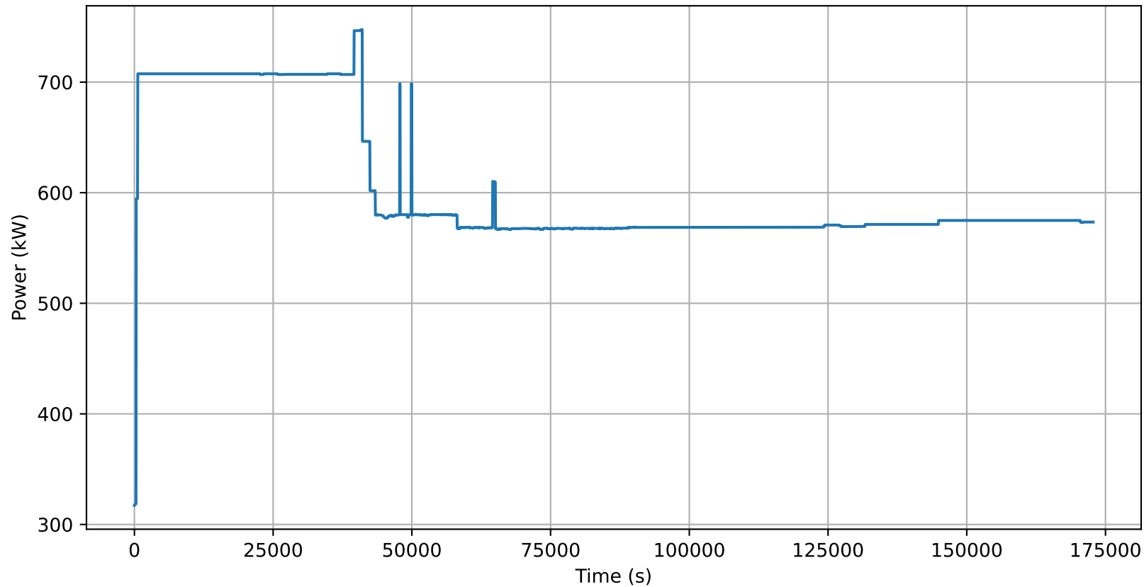
Power History
