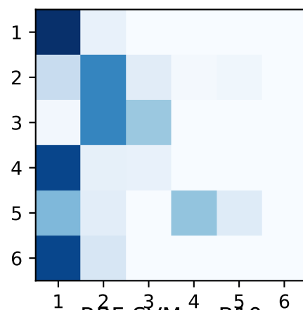
RBF-SVM — B10
