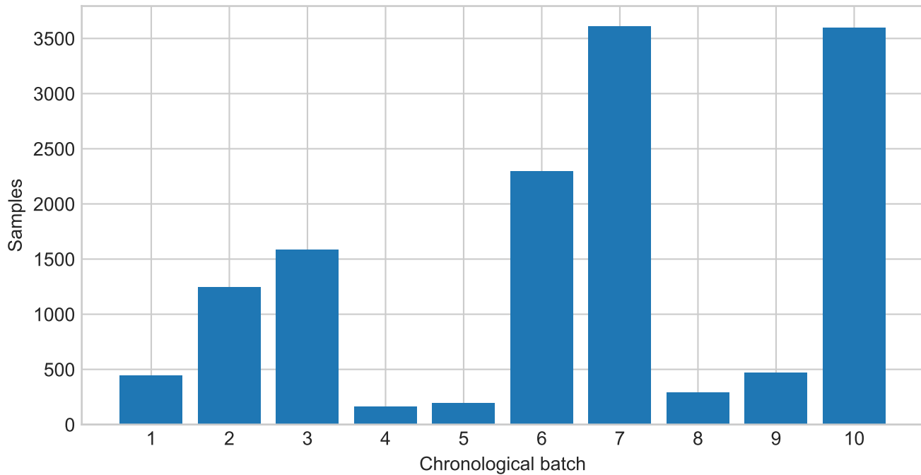
Dataset chronology
