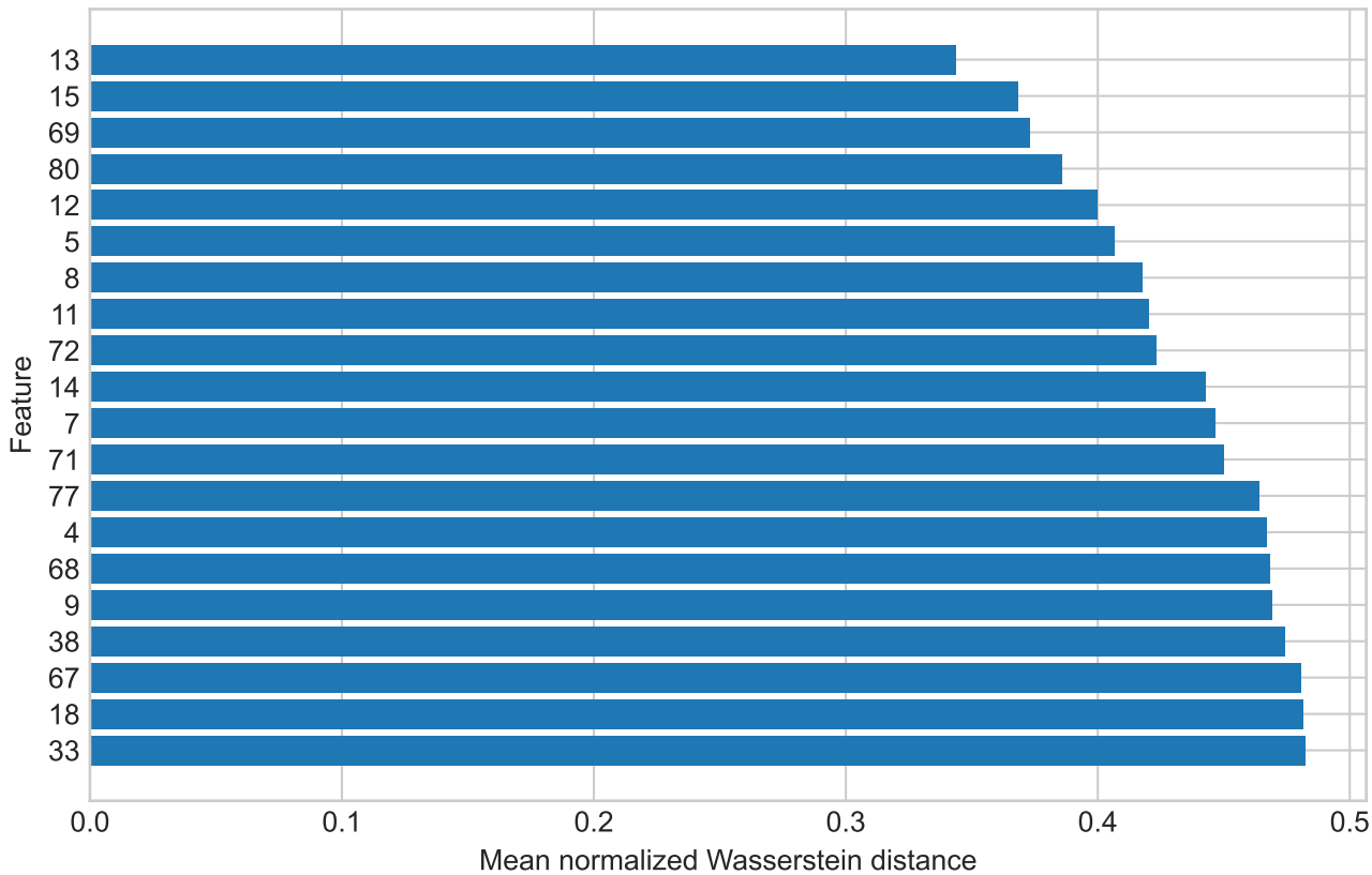
Top 20 stable features
