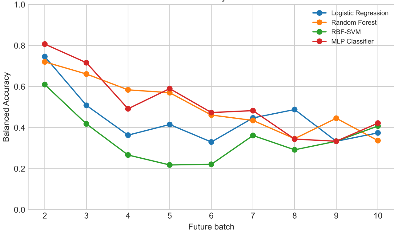
Balanced Accuracy Across Drift
