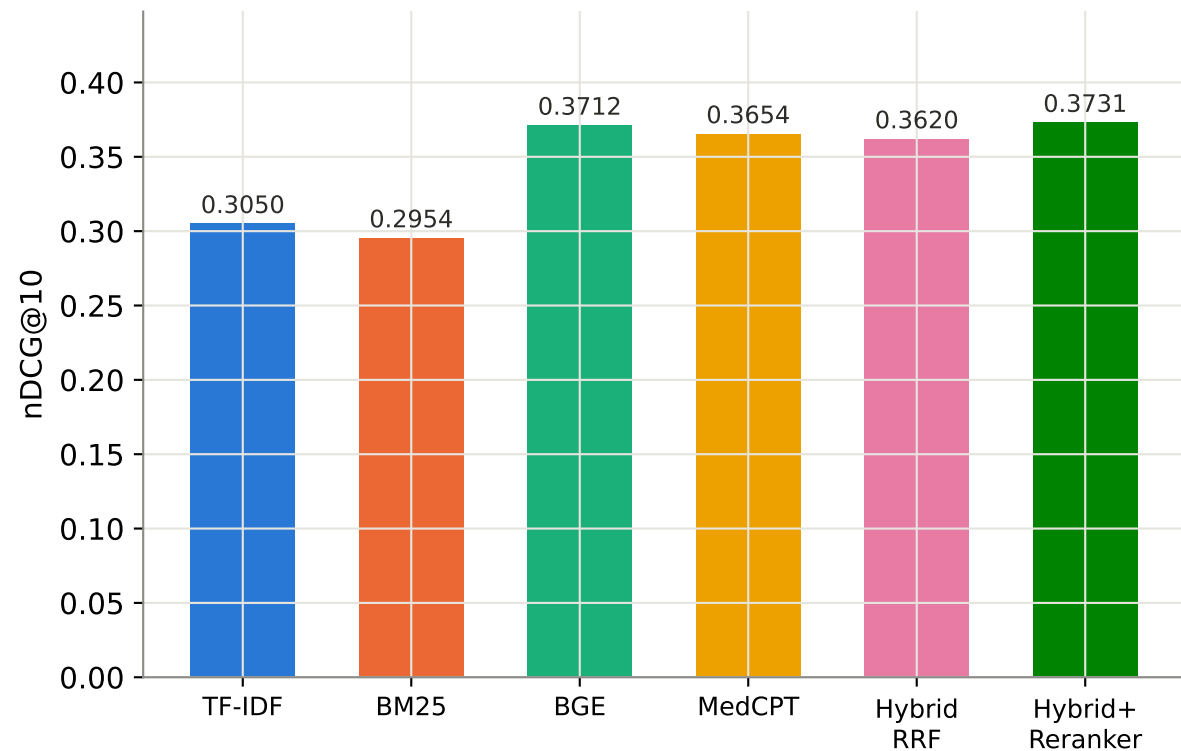
nDCG@10 by model (test split, n=323)
