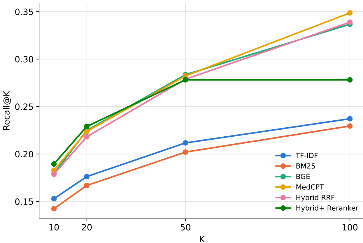
Recall@K curves, all six models (real test-split results)
