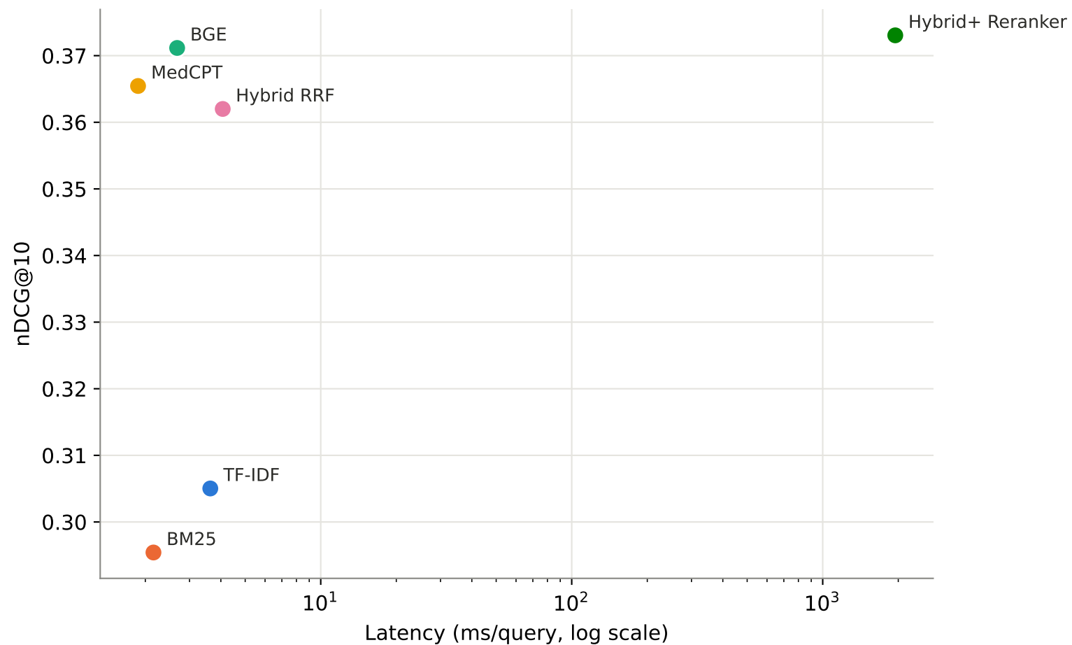
Effectiveness vs. efficiency: nDCG@10 vs. latency (real measurements)
