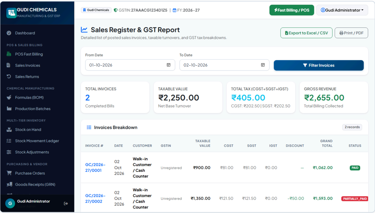
Figure 8.1: Sales & GST Analytics Report with Date Filtering and Excel Export
