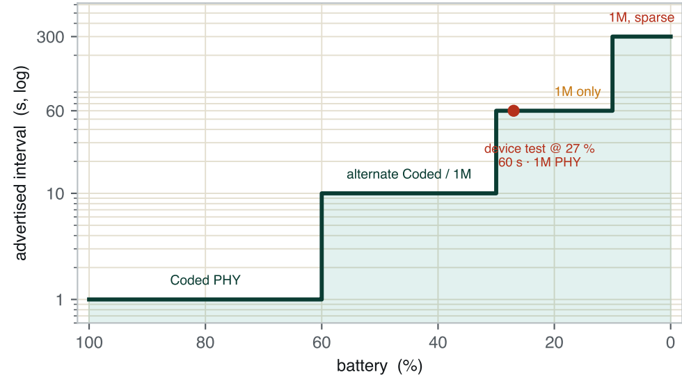
B · Battery-adaptive duty cycle (measured, Realme 7)
