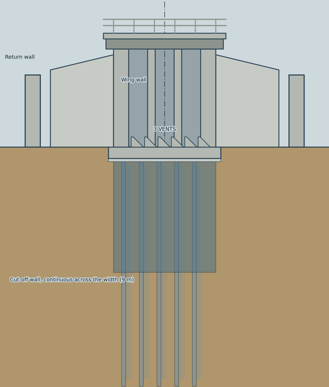
REGULATOR - CONSTRUCTION SEQUENCE FRONT RIVER SIDE ELEVATION | STAGE 09/11 Bridge deck and hoist platform
