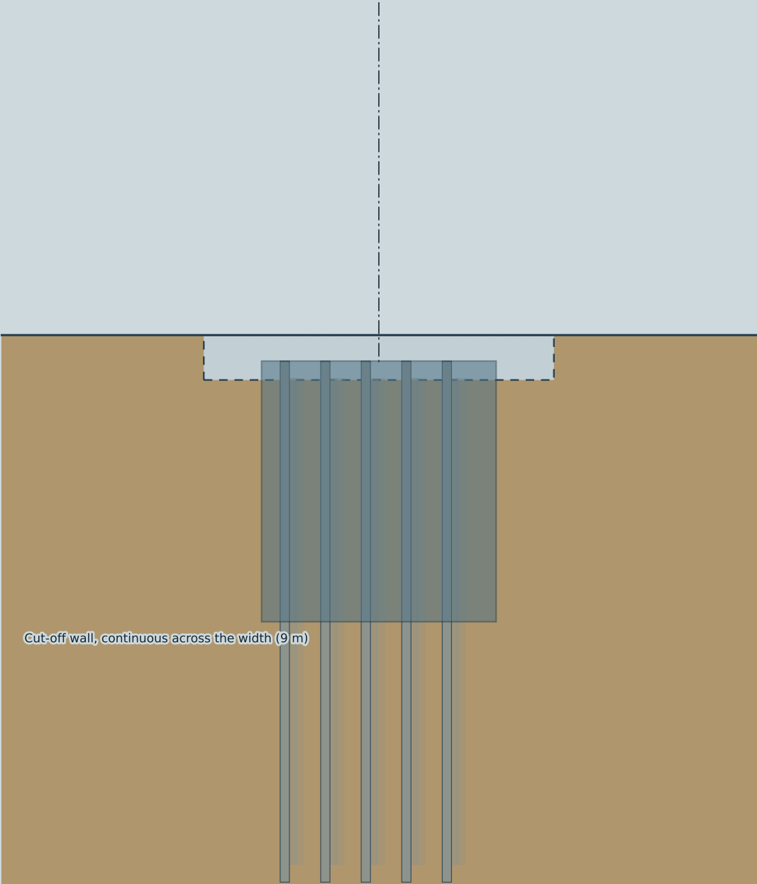
REGULATOR - CONSTRUCTION SEQUENCE FRONT RIVER SIDE ELEVATION | STAGE 04/11 U-type sheet piles
