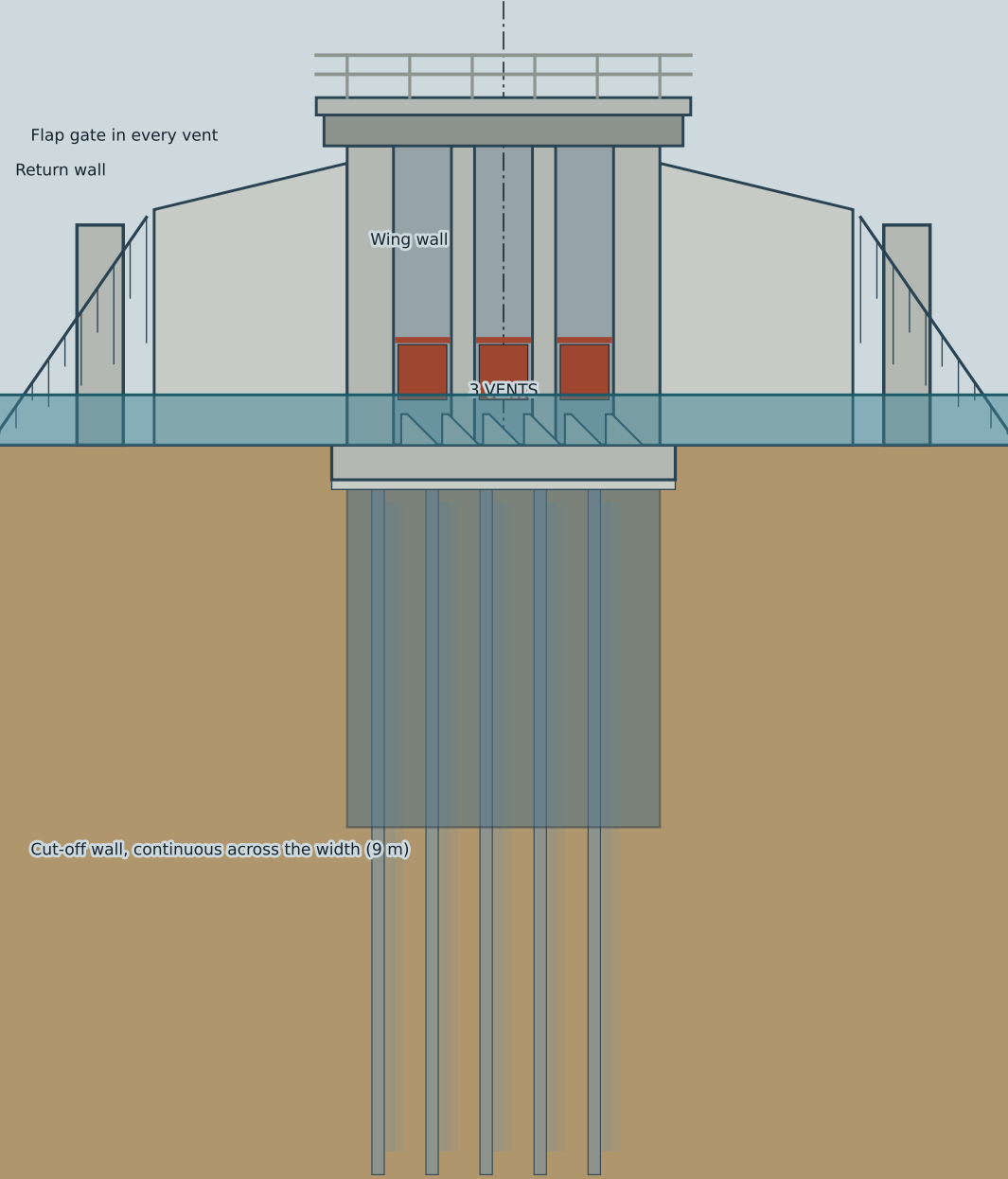
REGULATOR - CONSTRUCTION SEQUENCE FRONT RIVER SIDE ELEVATION | STAGE 11/11 Backfilling and trial operation
