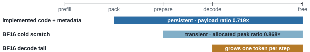
Figure 4: Decode path and allocation lifetime. Two homogeneous FlashInfer calls are merged through log-sum-exp state; the coded payload persists while BF16 cold scratch is live during decode.
