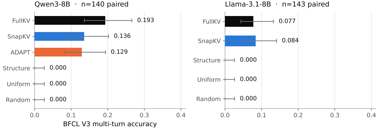
Figure 10. Paired BFCL accuracy with Wilson intervals. The same ordering holds on both models: FullKV and attention selection are indistinguishable, while the three non-attention policies are at zero with a Wilson upper bound of 0.027.
