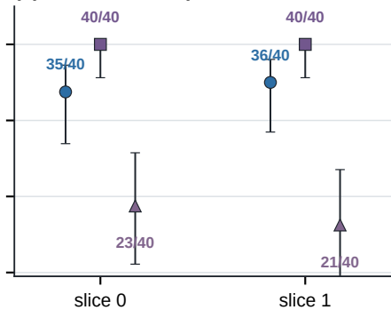
(b) Llama 5%: SnapKV wins both
