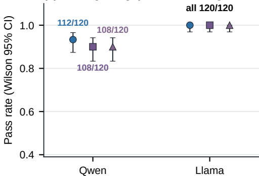
(a) 25%: Qwen gap, Llama ceiling
