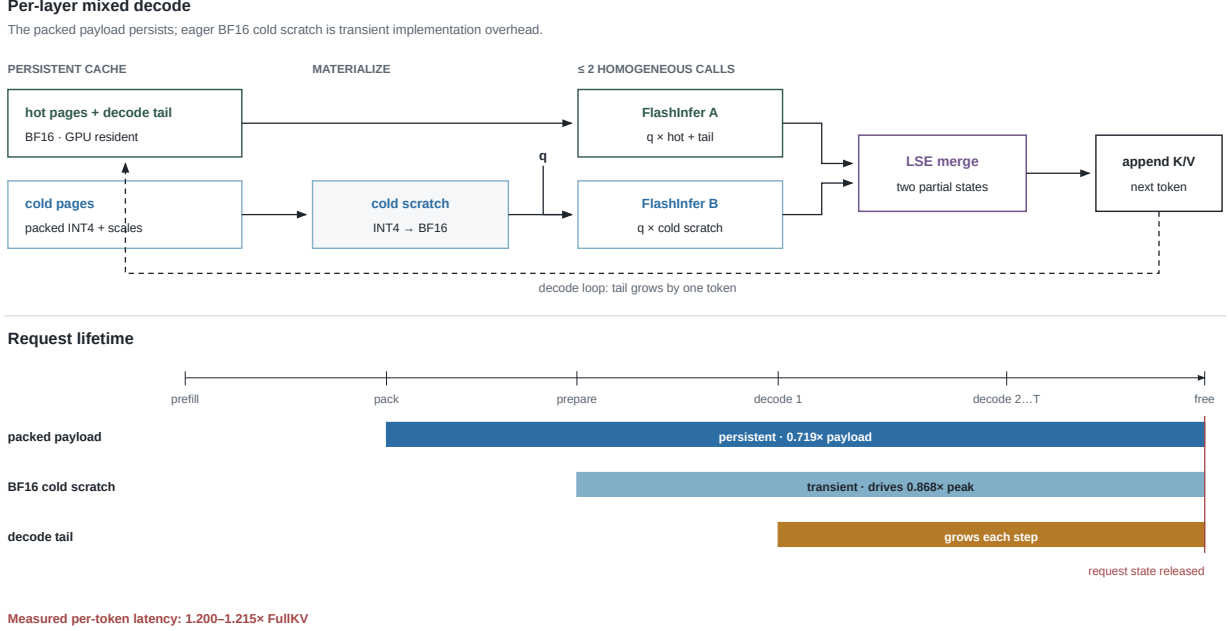
Figure 4. Decode path and allocation lifetime. Two homogeneous FlashInfer calls are merged through log-sum-exp state; packed payload persists while BF16 cold scratch is live during decode.
