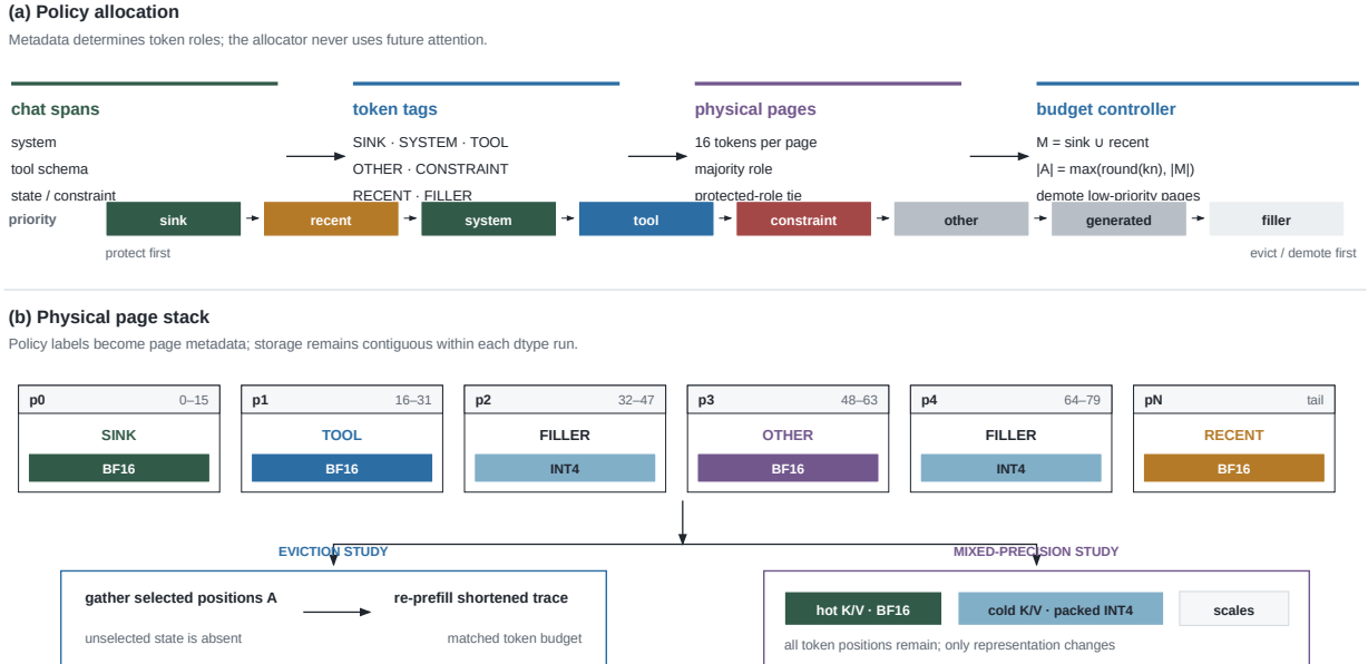
Figure 3. PriorityKV architecture. Chat metadata becomes token roles and 16-token pages before matched-budget retention or precision placement. The page records are illustrative.
