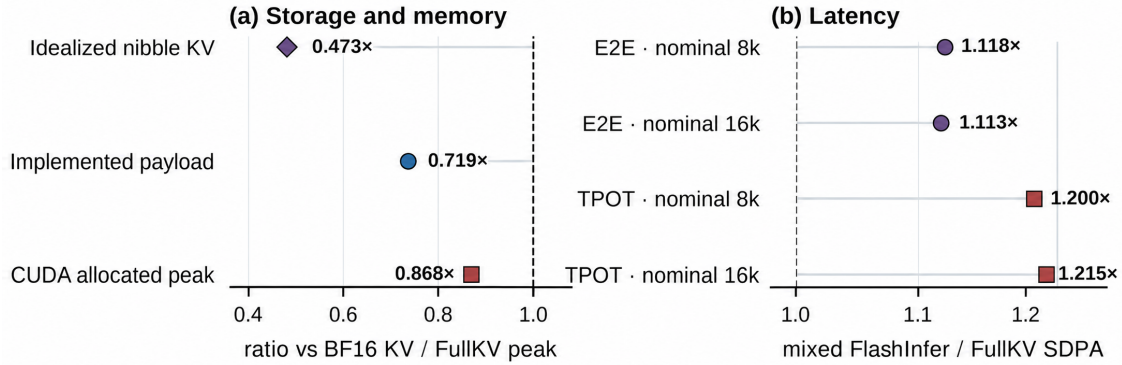
Figure 5: Storage trade-off on H200. The implemented code-plus-metadata payload is smaller than the FullKV cache, while the allocated peak falls less because cold pages are expanded into BF16 scratch for attention. Latency compares the mixed FlashInfer path against FullKV SDPA; the dashed line marks parity.
