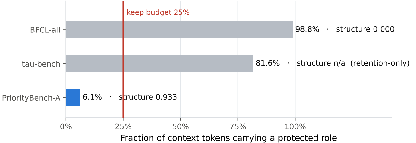
Figure 9: Protected mass relative to the keep budget. PriorityBench-A is 94.9% filler, so 6.1% of tokens carry a protected role and the policy has ample room to rank within a 25% budget. A BFCL system prompt is 32 JSON tool schemas, so 98.8% of tokens carry the protected TOOL role and nothing is available to discard. \tau -bench sits between at 81.6%; it is a retention-only audit and has no task-success value.
