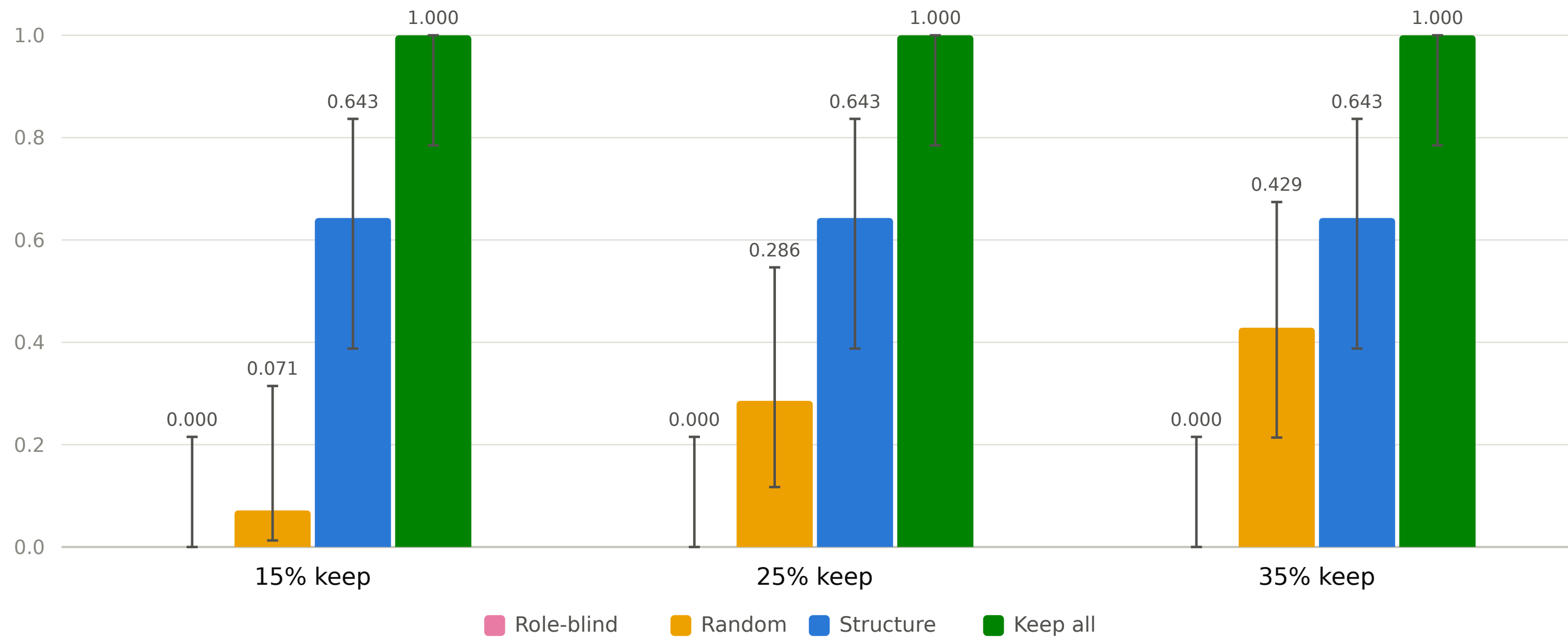
PriorityBench score
