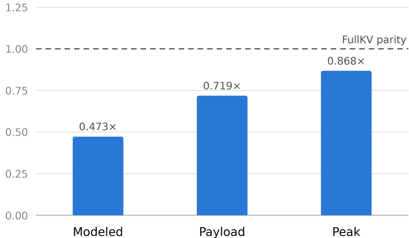
KV memory, ratio to FullKV (lower is better)
