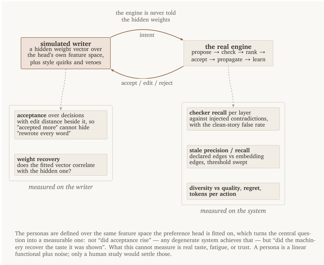
Figure 6: The loop and where the measurements are taken. Metrics on the left are properties of the writer’s behaviour; on the right, properties of the system.
