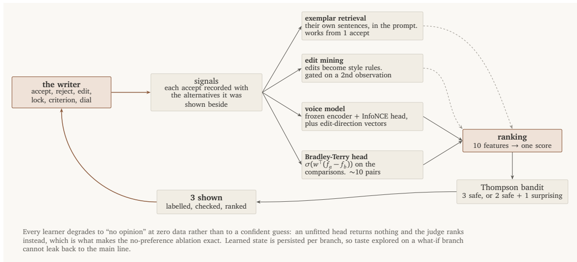
Figure 5: The loop. Every learner degrades to “no opinion” at zero data rather than to a confident guess, which is what makes the no-preference ablation exact. Learned state is persisted per branch, so taste explored on a what-if branch cannot leak back to the main line.
