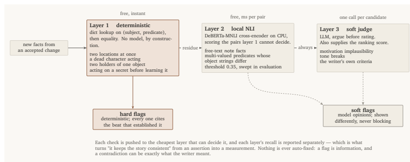
Figure 2: The checker. Layer 1 is deterministic and, by construction, cannot call a model: it imports nothing from the provider layer, and a test parses its imports to prove it. Layer 2 handles only the residue layer 1 cannot decide. Layer 3 is an opinion, labelled as one.
