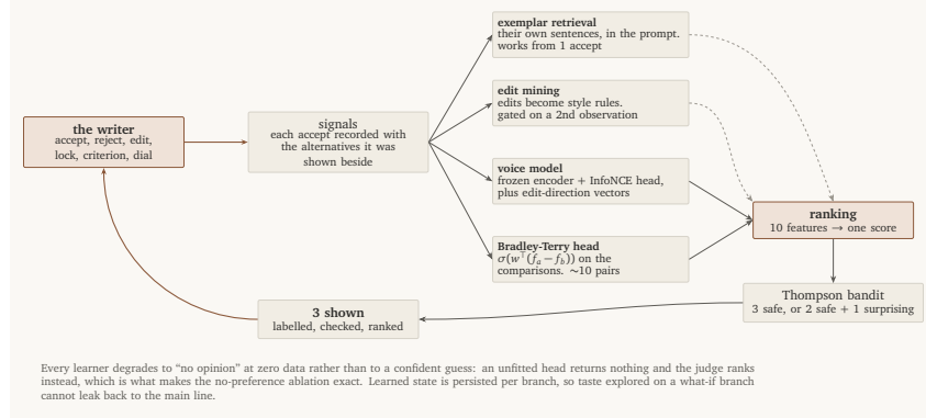
Figure 3: The loop. Every learner degrades to “no opinion” at zero data rather than to a confident guess, which is what makes the no-preference ablation exact. Learned state is persisted per branch, so taste explored on a what-if branch cannot leak back to the main line.
