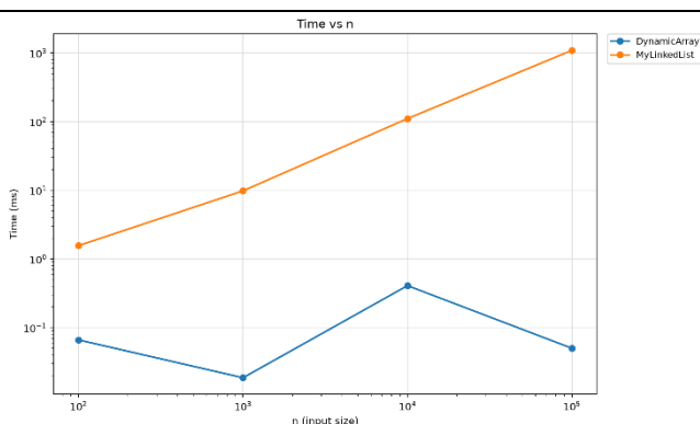
Figure 1. W1: indexed access time.
