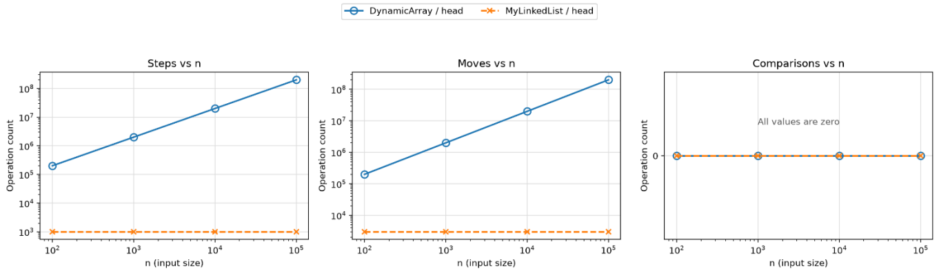
Figure 7. W3: operation counts for head updates.
