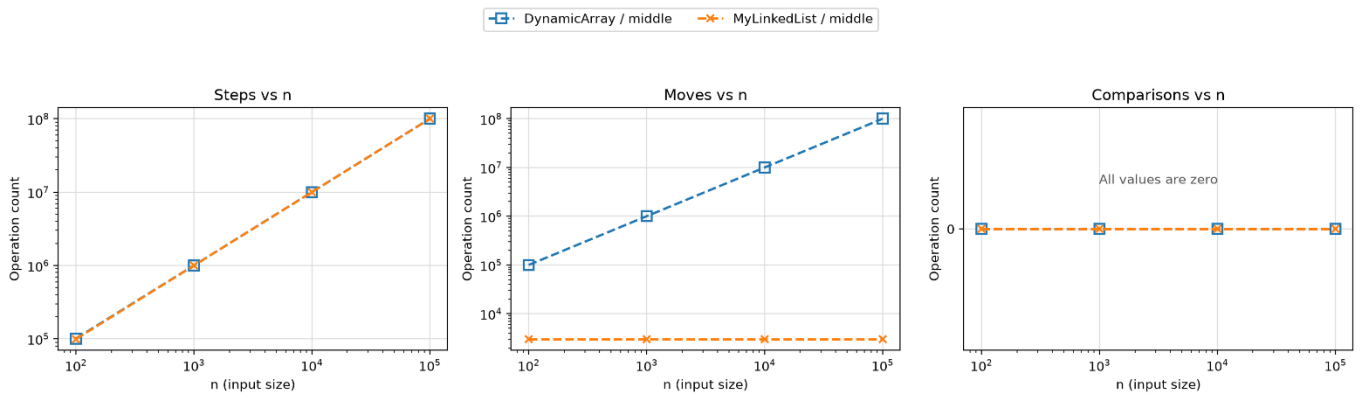
Figure 8. W3: operation counts for middle updates.
