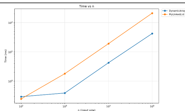
Figure 2. W2: search time.
