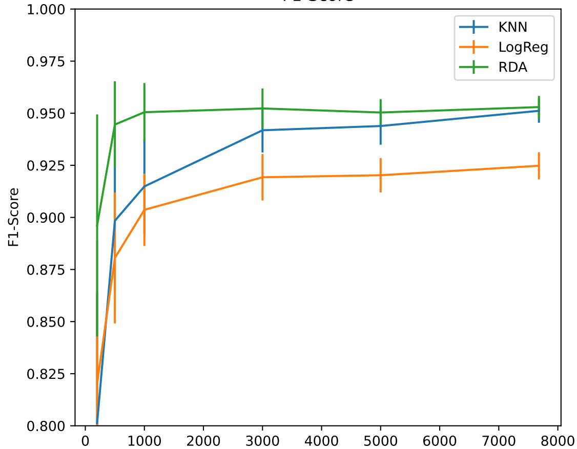
F1-Score
