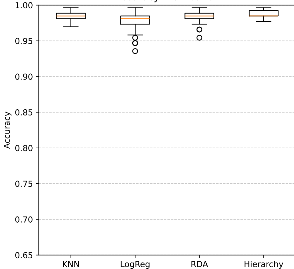
Accuracy Distribution
