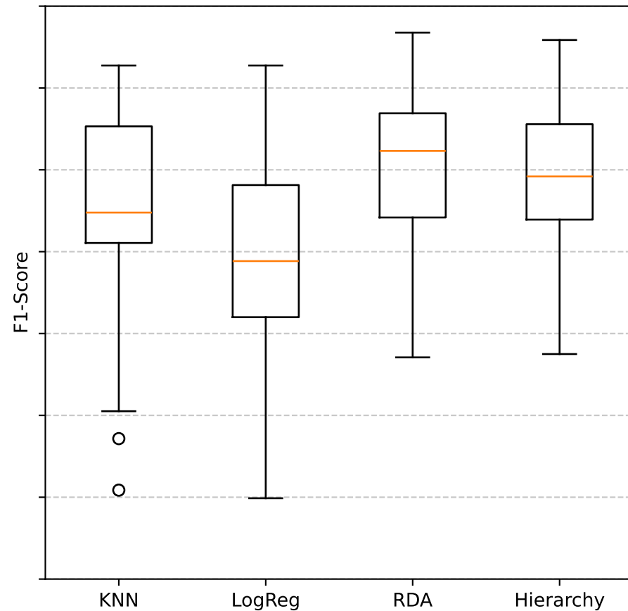
F1-Score Distribution
