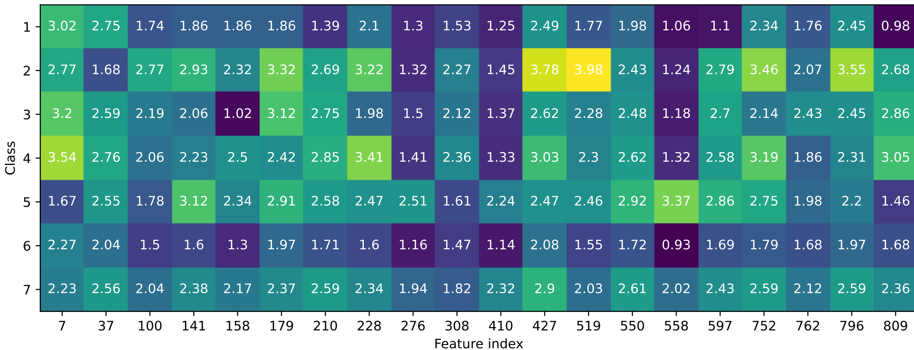
Variance of features between classes
