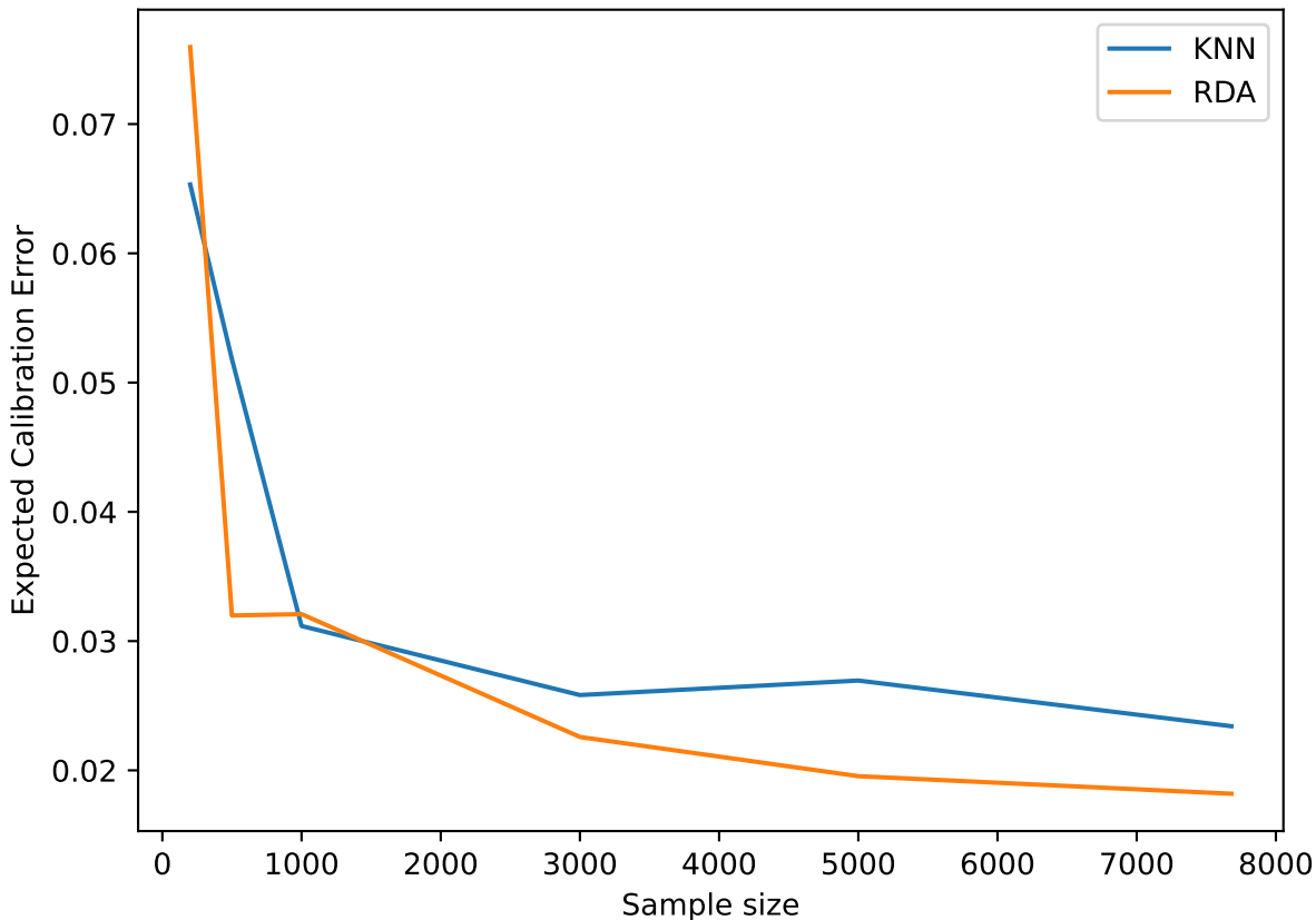
Expected Calibration Error over Sample Size
