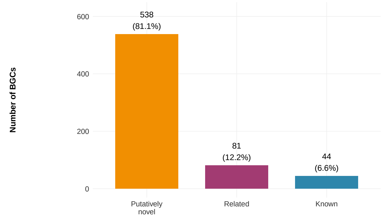
MIBiG-based novelty classification
