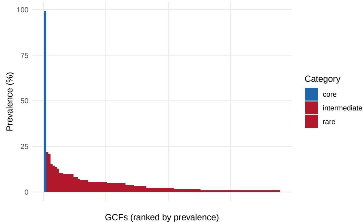
GCFs ranked by prevalence (c0.7)
