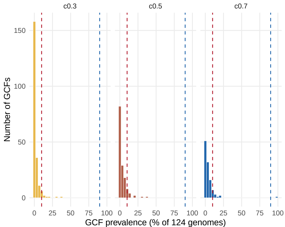
GCF prevalence distribution across cutoffs
