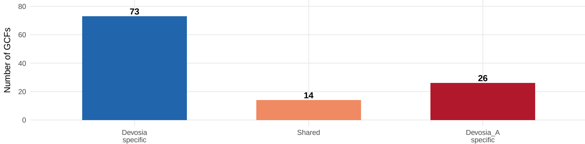
Devosia vs Devosia_A (c0.7)
