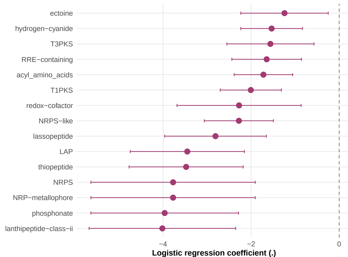
B Significant class associations (FDR<0.05)
