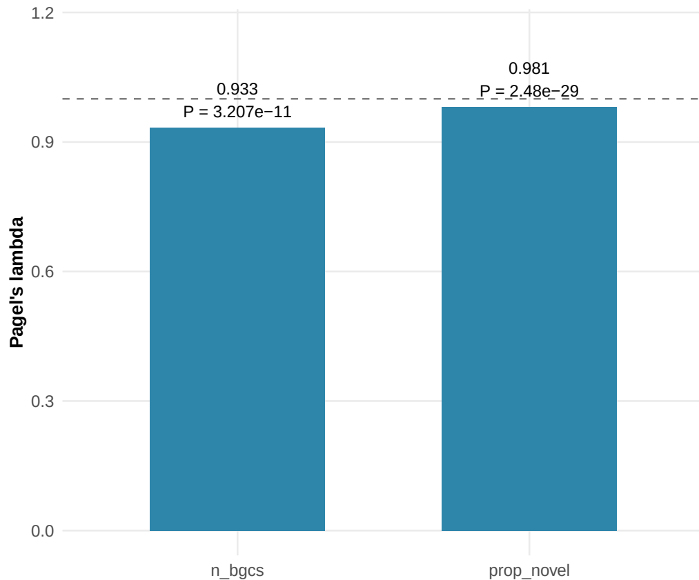
A Phylogenetic signal
