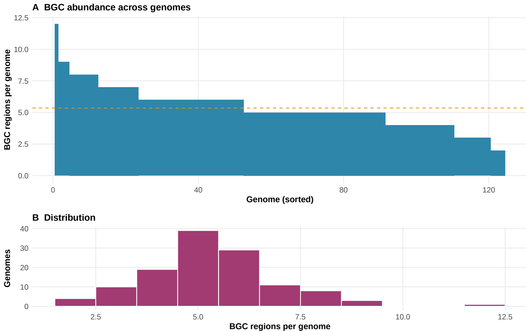
Figure 2. BGC abundance across Devosia genomes
