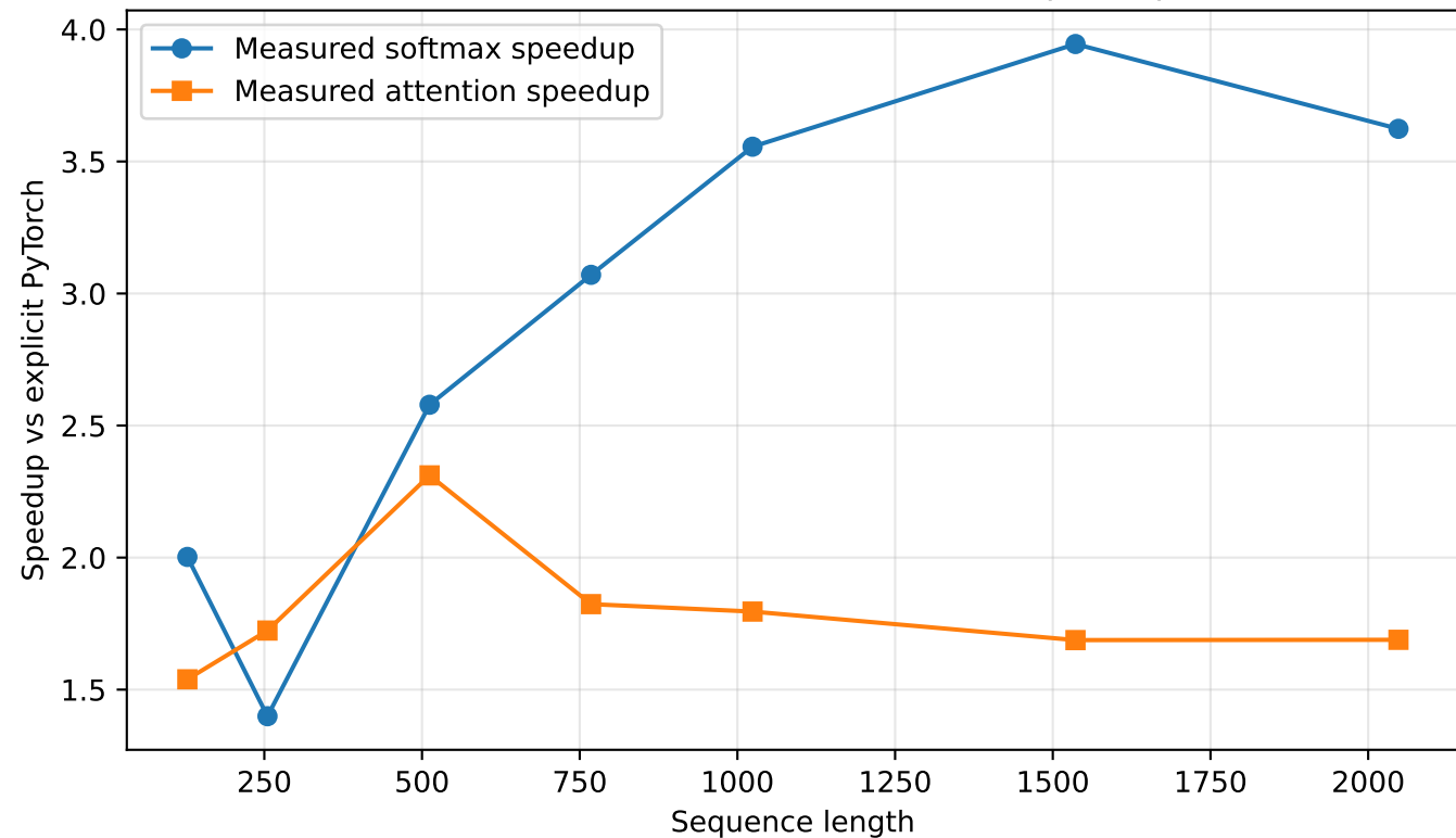
Kernel versus end-to-end attention speedup
