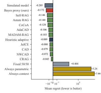
(b) Per-baseline regret (symlog); same ordering visualized.
