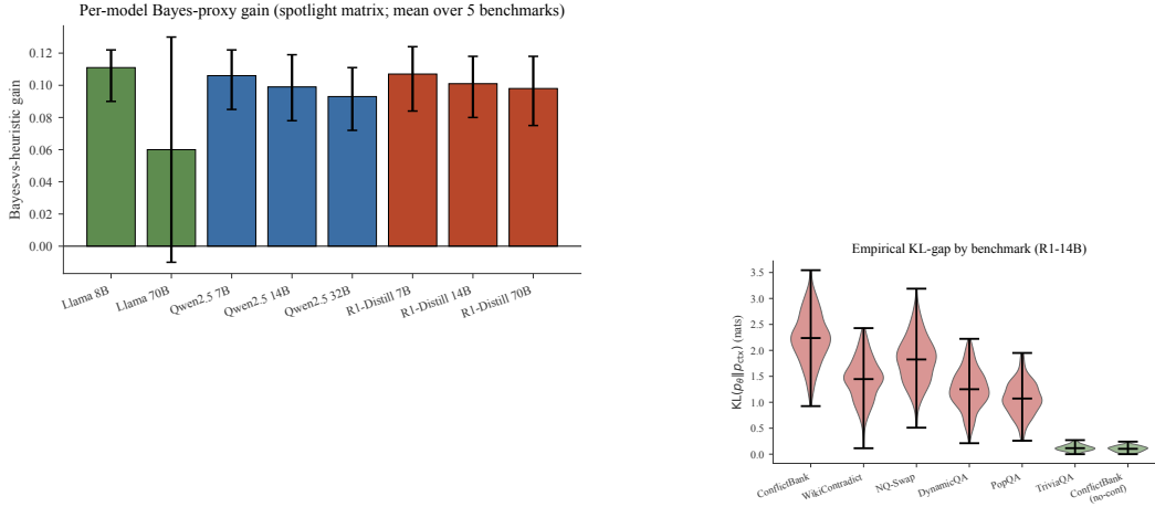
Figure 3: Per-model and per-benchmark structure. Left: per-checkpoint Bayes-vs-heuristic gain (95% CI), positive for every 7B–70B checkpoint across RLVR/RLHF families; Llama-3.1-70B alone shows +0.060 over the heuristic. Right: per-benchmark KL gap KL(p_\theta || p_{ctx}) on R1-14B; conflict slices \geq 1 nat, controls \sim 0.1 nat.
