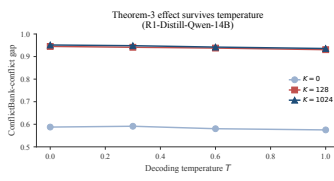
Figure H.10: Temperature robustness. Conflict gap survives all four decoding temperatures.
