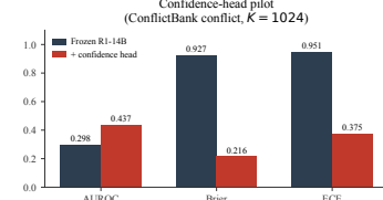
Figure H.11: Confidence-head pilot. AUROC/Brier/ECE improve on worst slice; accuracy unchanged.
