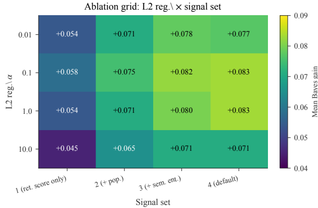
Figure J.13: Two-axis ablation grid. Mean Bayes-vs-heuristic gain as a function of L2 regularization \alpha and signal set size. Optimum at \alpha = 0.1 , 4 signals. The default \alpha = 1.0 is within 0.001 of the optimum.
