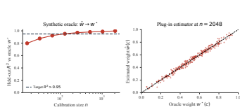
Figure H.9: Oracle convergence. Held-out R^2(\hat{w}, w^*) = 0.998 at n = 2048 .
