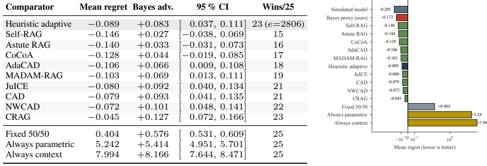
Figure 2: Spotlight comparison against named baselines. Left: per-baseline statistics (25-cell paired bootstrap, sign test, fixed- \lambda e-value); BAYESARBITER mean regret -0.172 . Right: same ordering on a symlog regret axis. 25-cell CIs clear zero against 7 of 10 named methods (heuristic-adaptive +0.083 , plus AdaCAD/MADAM-RAG/JulCE/CAD/NWCAD/CRAg); the four tightest (AdaCAD, CoCoA, Astute, Self-RAG) clear zero on the powered n=210 design at +0.064/ +0.043/ +0.032/ +0.022 (Section 4.1).
