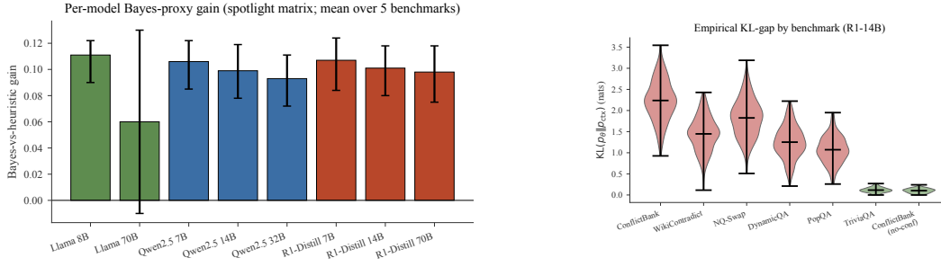
Figure 3: Per-model and per-benchmark structure. Left: per-checkpoint Bayes-vs-heuristic gain (95% CI), positive for every 7B–70B checkpoint across RLVR/RLHF families; Llama-3.1-70B alone shows +0.060 over the heuristic. Right: per-benchmark KL gap KL(p_\theta || p_{ctx}) on R1-14B; conflict slices \geq 1 nat, controls \sim 0.1 nat.
