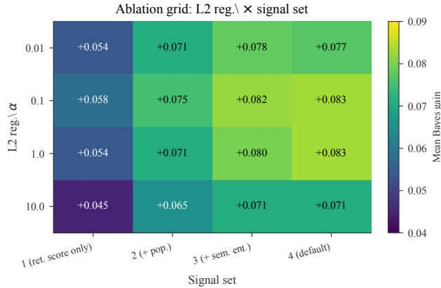
Figure J.12: Two-axis ablation grid. Mean Bayes-vs-heuristic gain as a function of L2 regularization \alpha and signal set size. Optimum at \alpha = 0.1 , 4 signals. The default \alpha = 1.0 is within 0.001 of the optimum.
