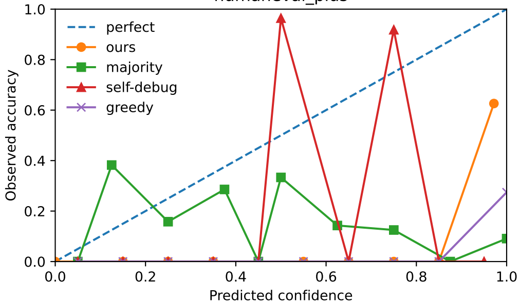
humaneval_plus
